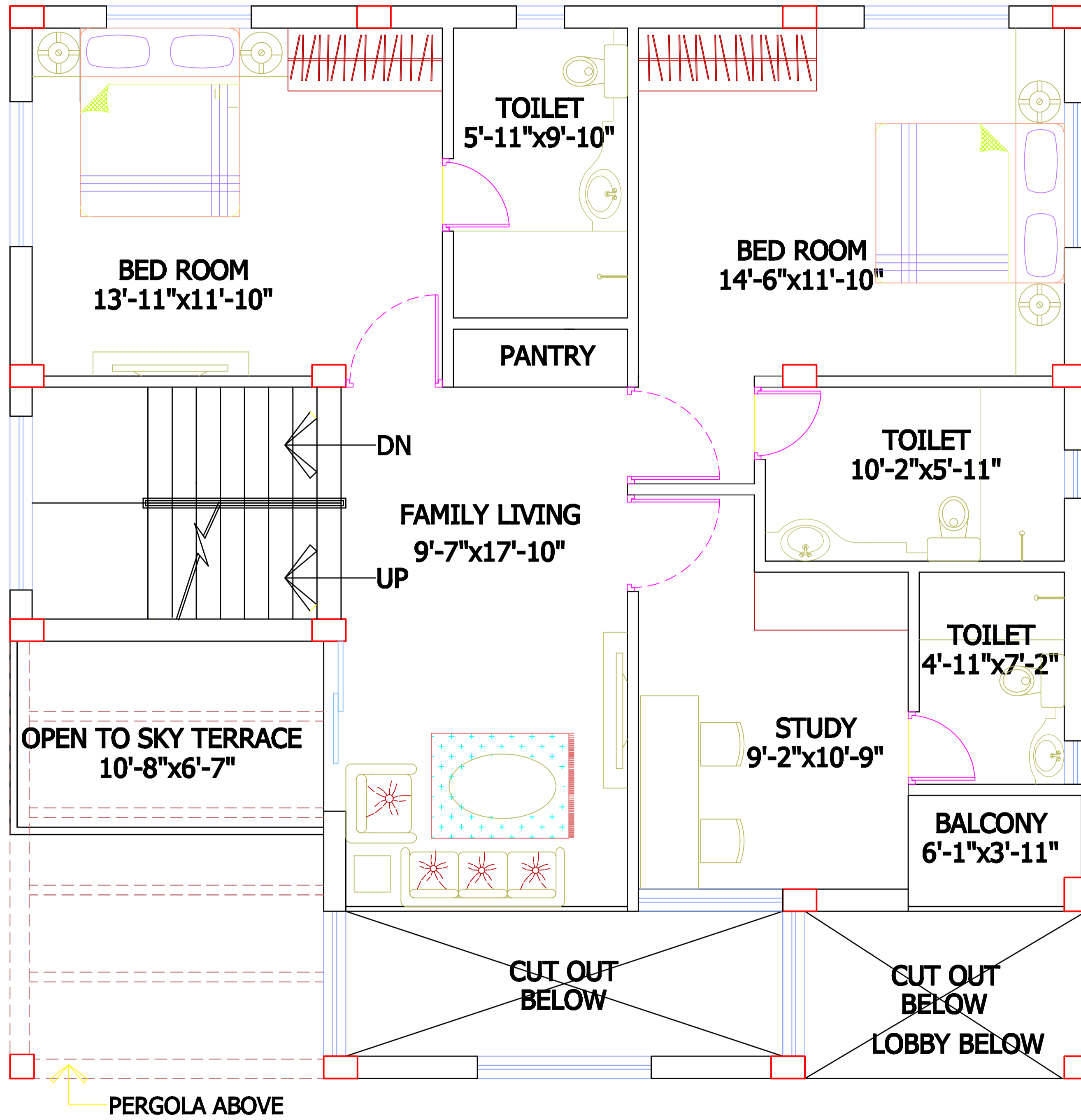
FIRST FLOOR PLAN BUNGALOW (VILLA) BV A 06
