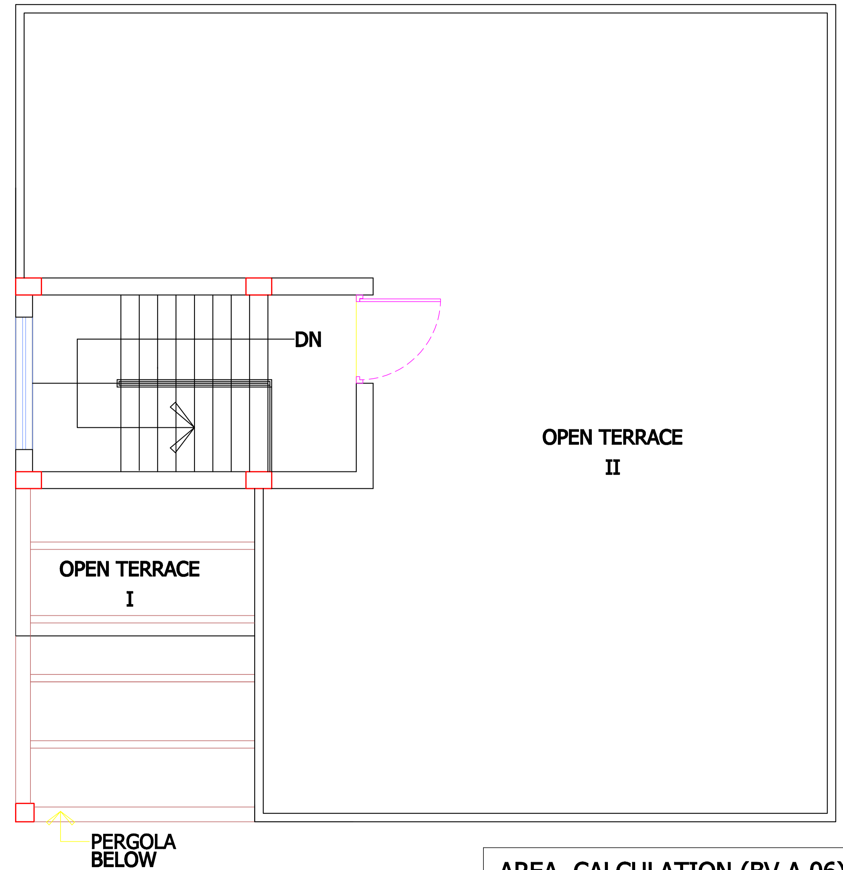
ROOF PLAN BUNGALOW (VILLA) BV A 06
