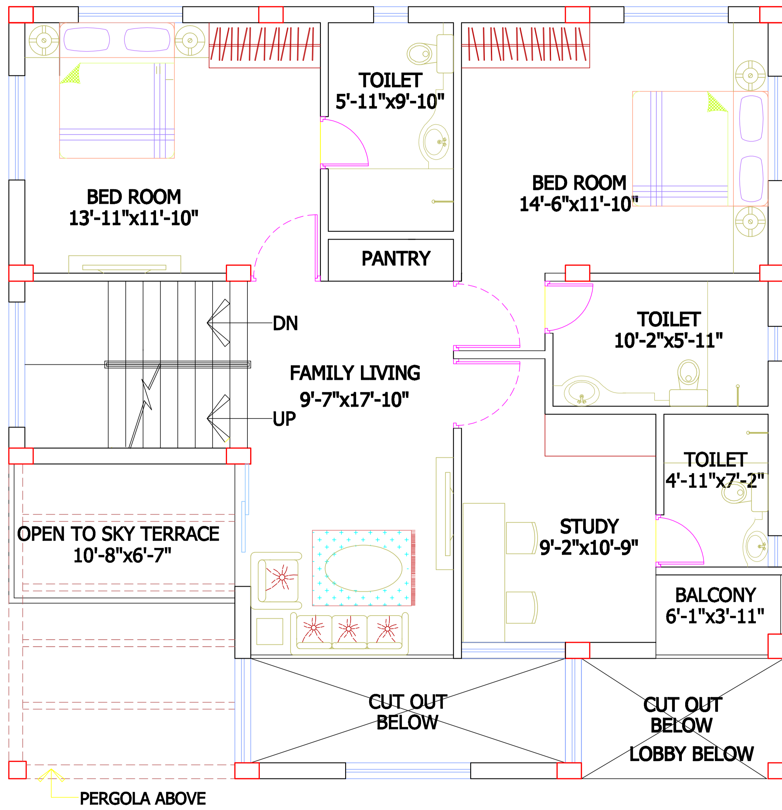
FIRST FLOOR PLAN BUNGALOW (VILLA) BV A 04
