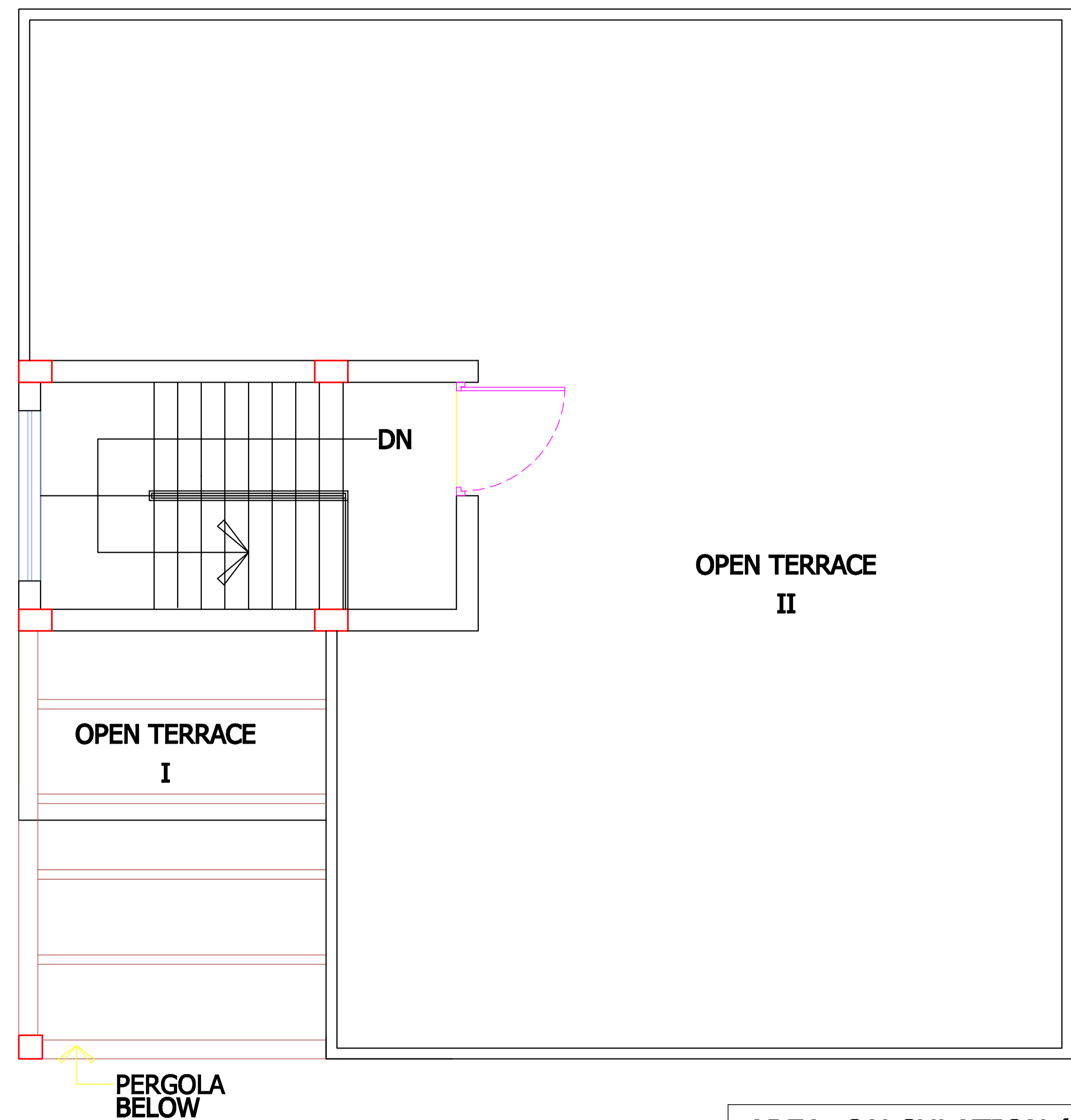
ROOF PLAN BUNGALOW (VILLA) BV A 04
