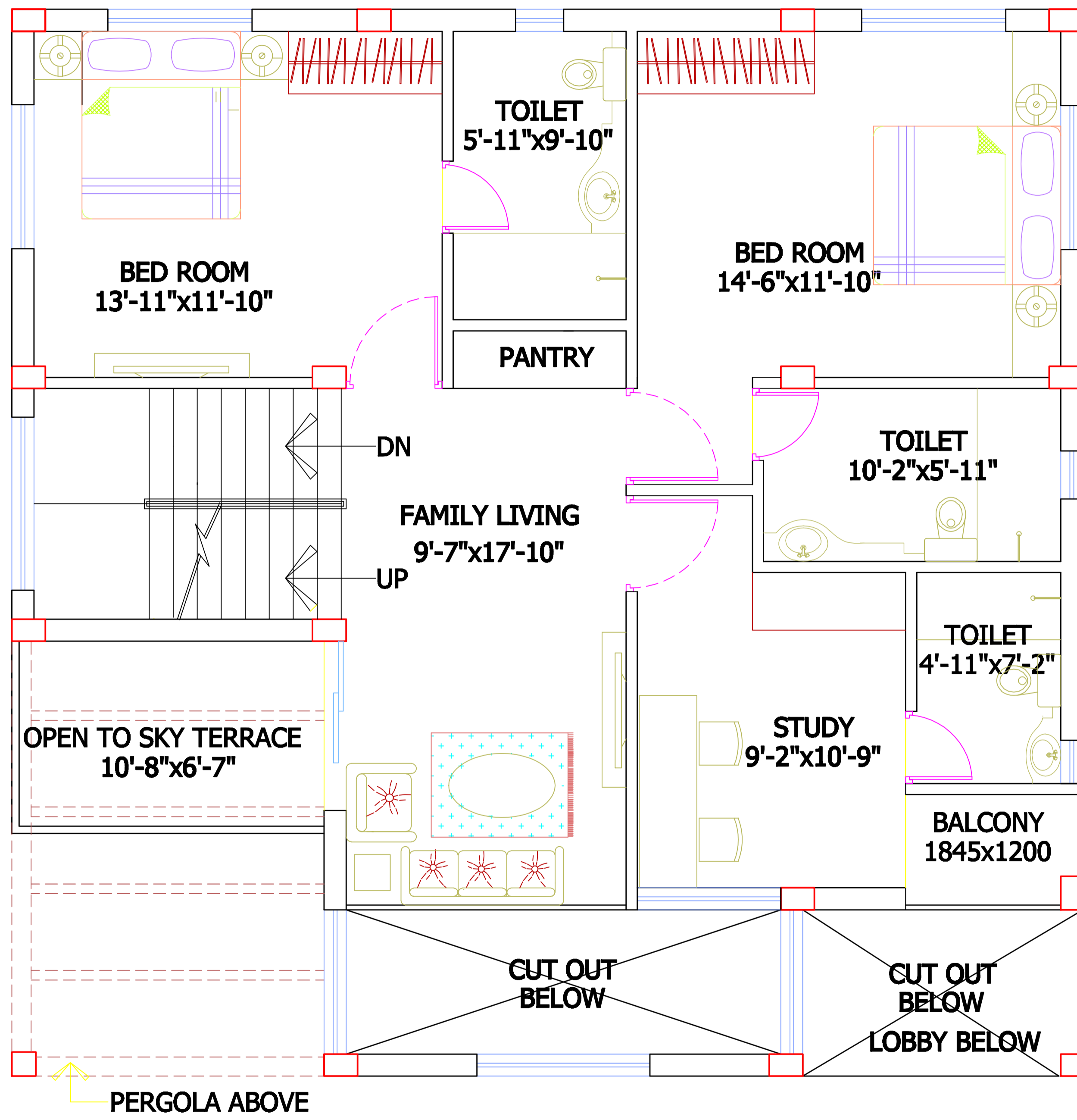
FIRST FLOOR PLAN BUNGALOW (VILLA) BV A 02
